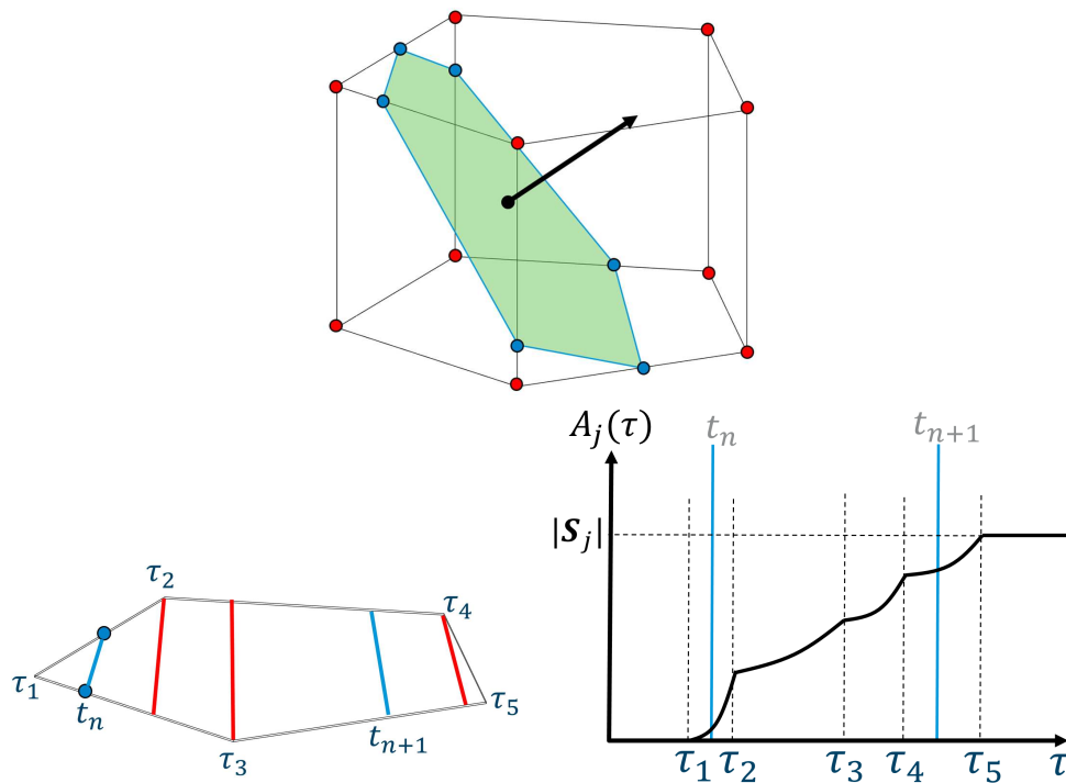
Figure 2. Calculation of the face flux using the isoAdvect scheme, [22].
